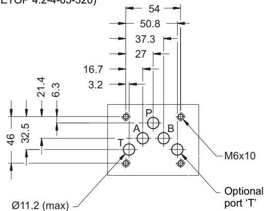
DL5BK* ISO 4401-05-04-0-05 (CETOP 4.2-4-05-320)
